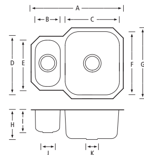
TRENT 1.5 bowl / Stainless Steel
